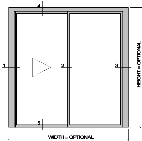
SCALE 1:10 (EXAMPLE OF A SLIDING-WINDOW, VERSION XO, SIZE 1000 X 1000 mm, VIEWED FROM OUTSIDE.)
