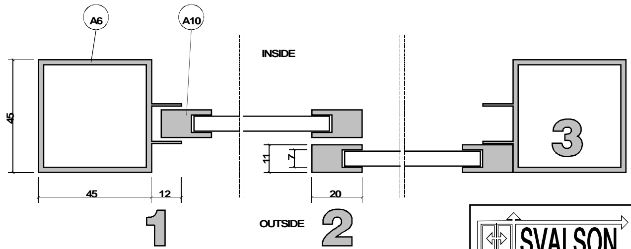
SCALE 1:10 (EXAMPLE OF A SLIDING-WINDOW, VERSION XO, SIZE 1000 X 1000 mm, VIEWED FROM OUTSIDE.)
