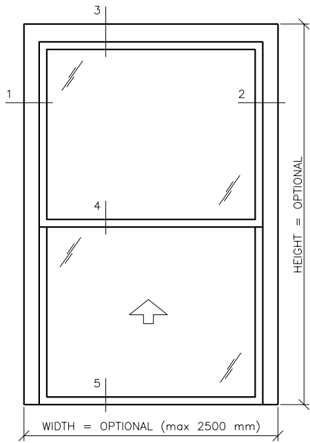
SCALE 1:10 (EXAMPLE OF A SLIDING WINDOW SIZE 1000 x 1500 mm, VIEWED FROM OUTSIDE.)
